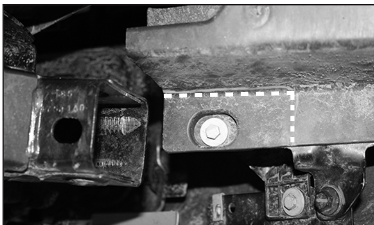
FIGURE 8 - STEP 5
