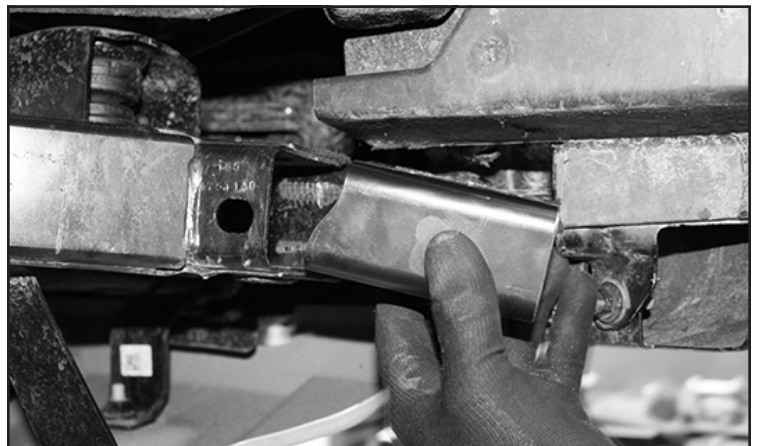
FIGURE 10 - STEP 6
