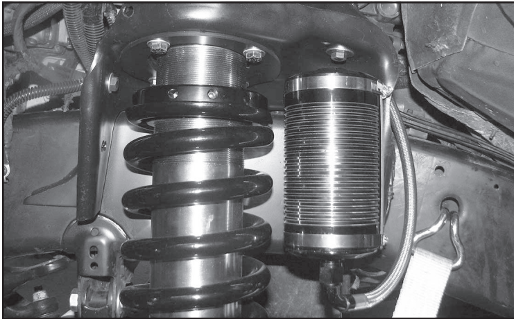
FIGURE 40 - STEP 25
