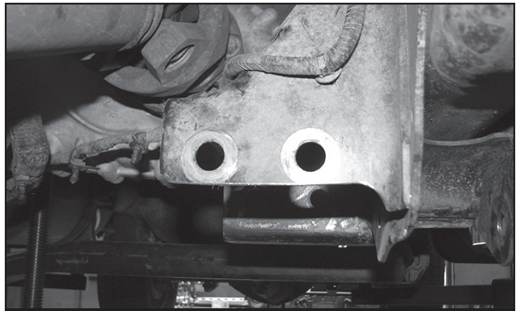
FIGURE 41 - STEP 41
