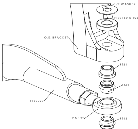
Front Upper Mount
