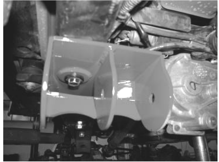
Factory Bolt in Rear Pocket
