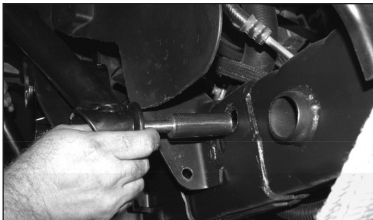
FIGURE 30 - STEP 26
