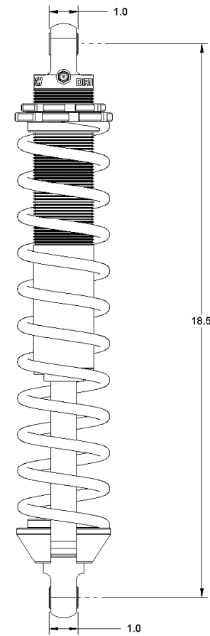
REAR SHORT SHOCK
