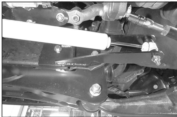
FIGURE 9 - STEP 7
