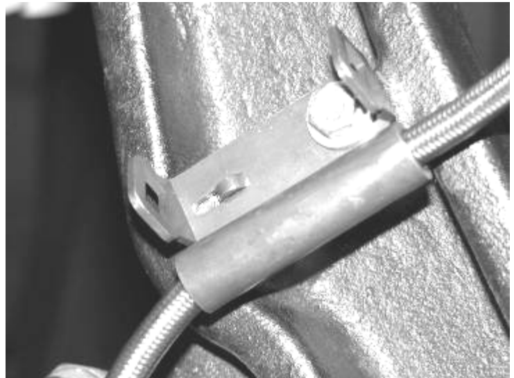
Photo shows brake lines on truck equipped with a Fabtech Long Travel Kit
