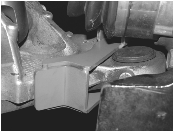
Photo of driver side Steering Stop (from front)
