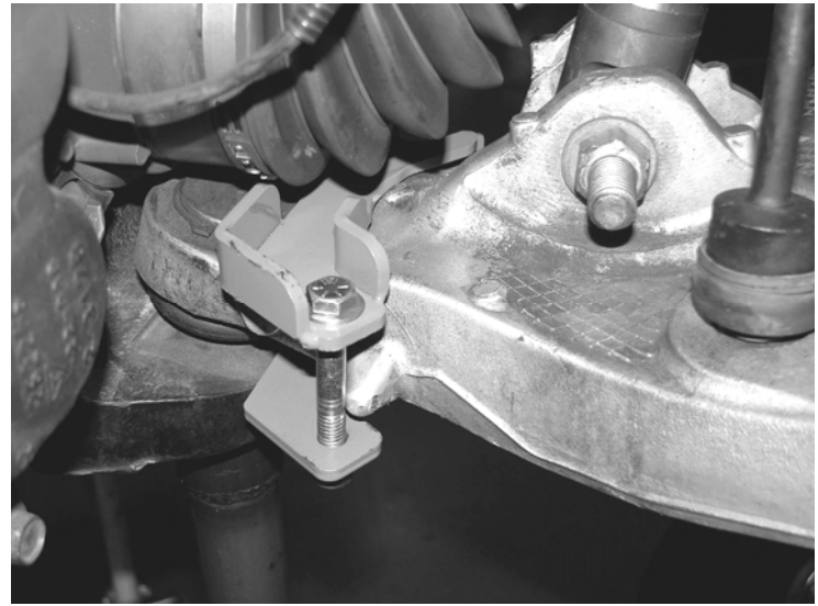
Photo of driver side Steering Stop (from rear)
