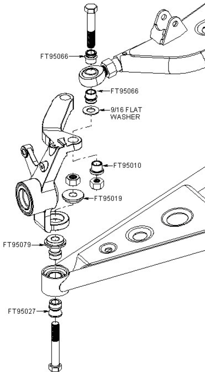
Upper and Lower Control Arm @ Knuckle
